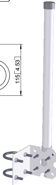
MOUNTS TO Ø 36 OMNI ANTENNAS VIA M6 U-BOLTS (MK4/A)
