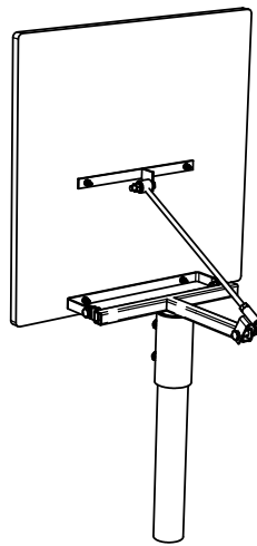
GROUND MOUNT
