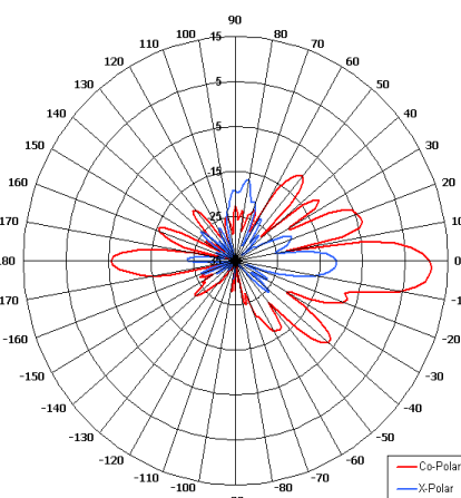
Elevation Pattern
