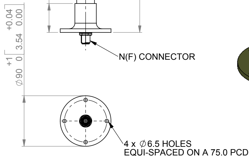
BASE VIEW
