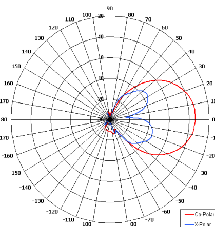
Elevation Pattern
