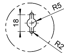
DETAIL A MOUNTING EYE 2 PLACES
