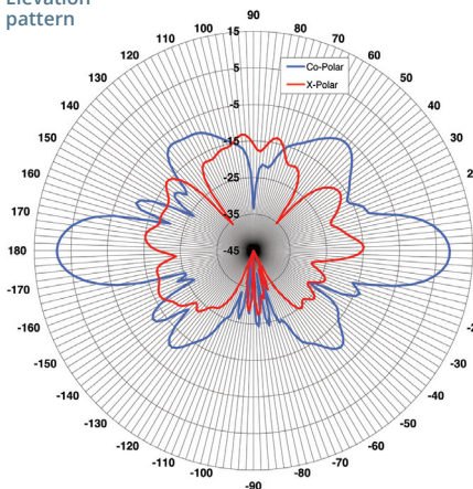
Elevation pattern
