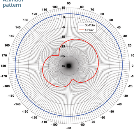
Azimuth pattern
