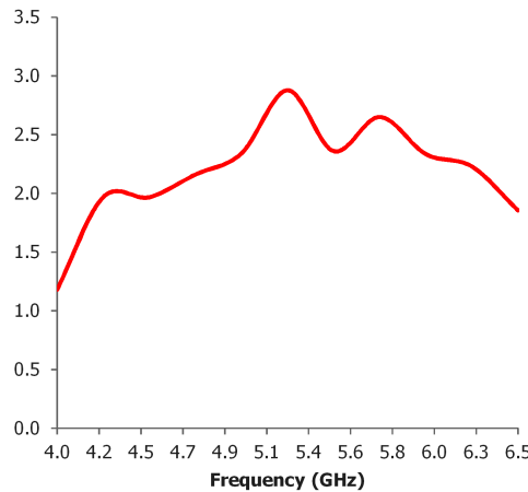
Gain Curve
