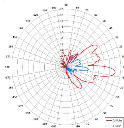
Elevation Pattern
