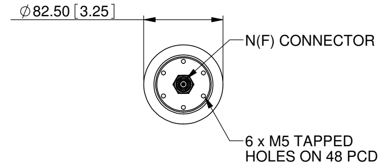
BASE VIEW
