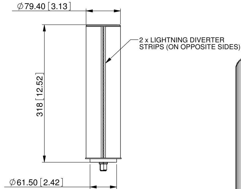
SIDE VIEW
