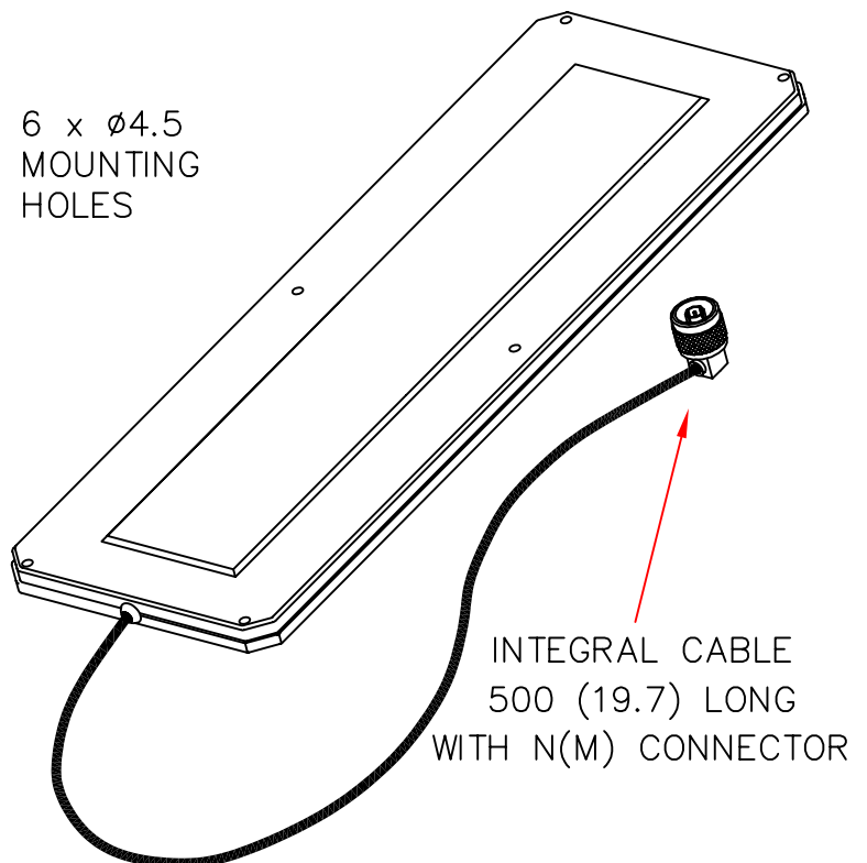
ISOMETRIC VIEW
