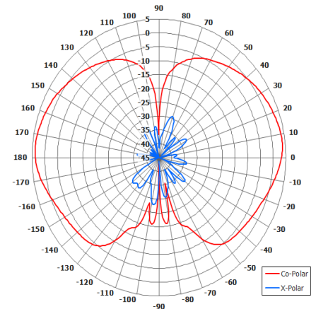
Elevation Pattern
