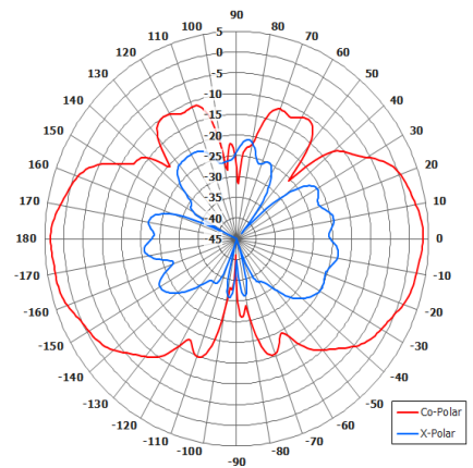
Elevation Pattern
