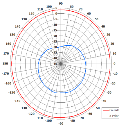
Azimuth Pattern
