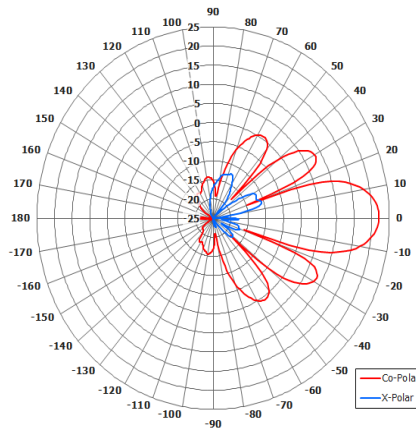
Azimuth Pattern
