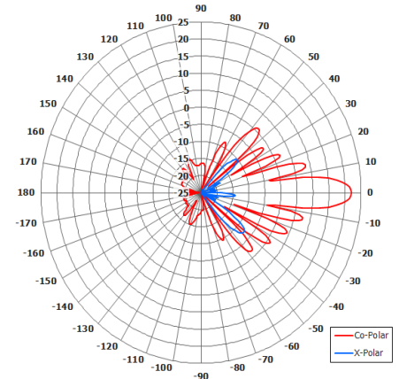
Elevation Pattern
