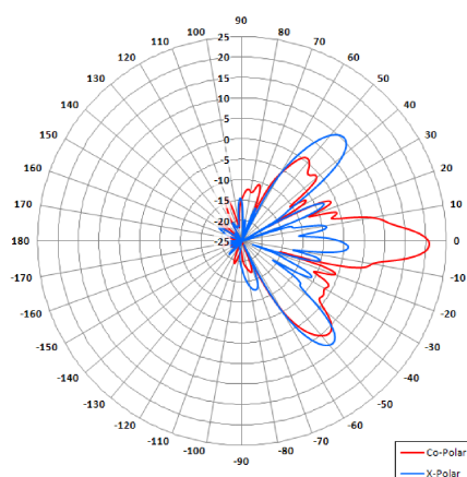
Elevation Polar Plot (similar product)
