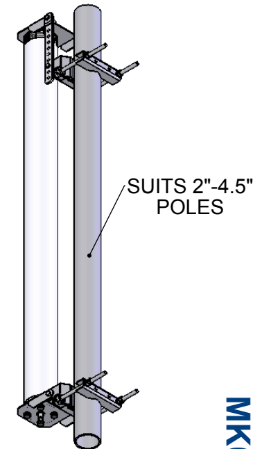
ISOMETRIC VIEW
