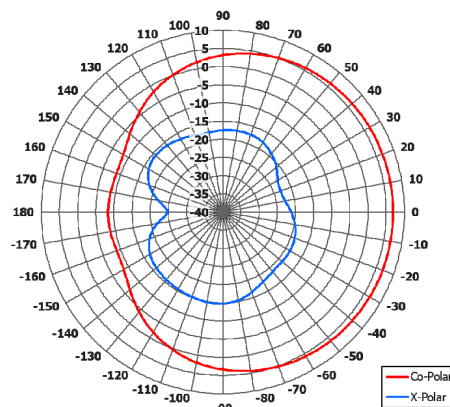
Azimuth Polar Plot (similar product)
