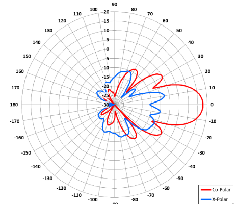
Elevation Polar Plot (similar product)
