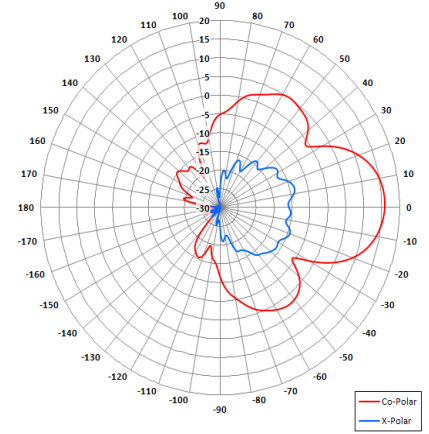
Elevation Pattern (similar product)
