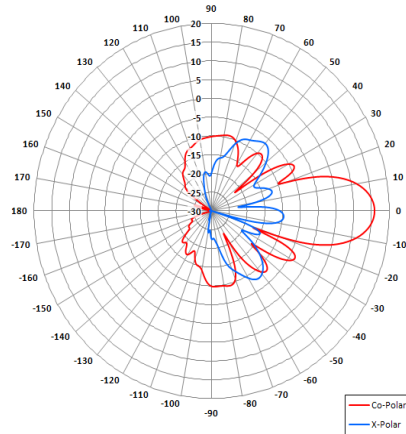
Azimuth Pattern (similar product)
