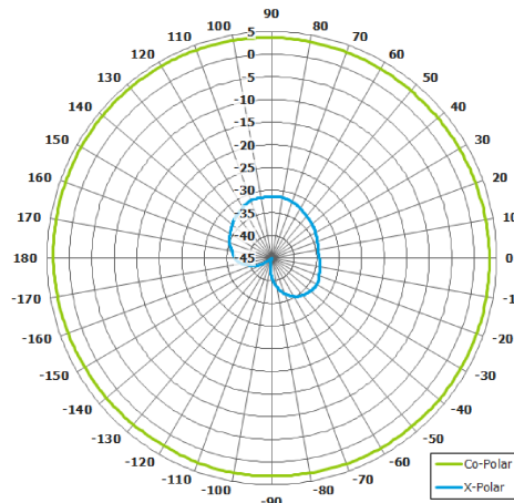
Azimuth Polar Plot (@ 915 MHz)
