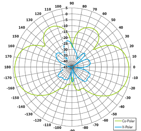
Elevation Polar Plot (@ 915 MHz)
