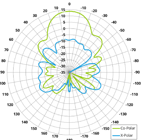
Elevation Polar Plot (@ 2.2 GHz)
