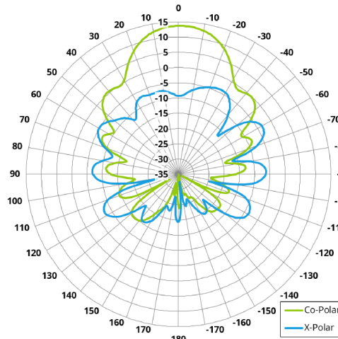
Azimuth Polar Plot (@ 2.2 GHz)
