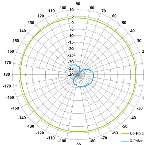
Azimuth Polar Plot (@ 2.3GHz)
