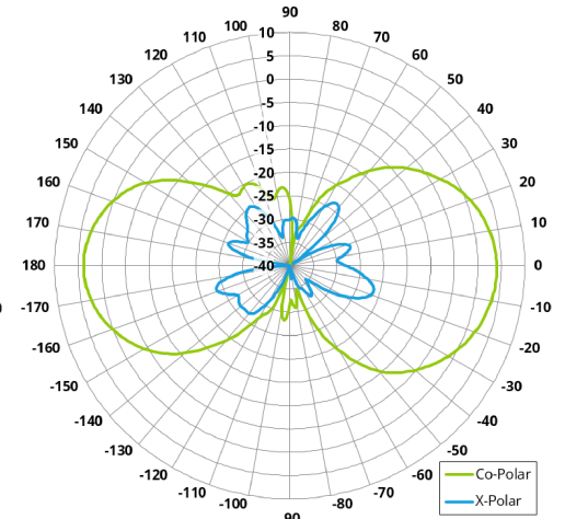
Elevation Polar Plot (@ 2.3GHz)
